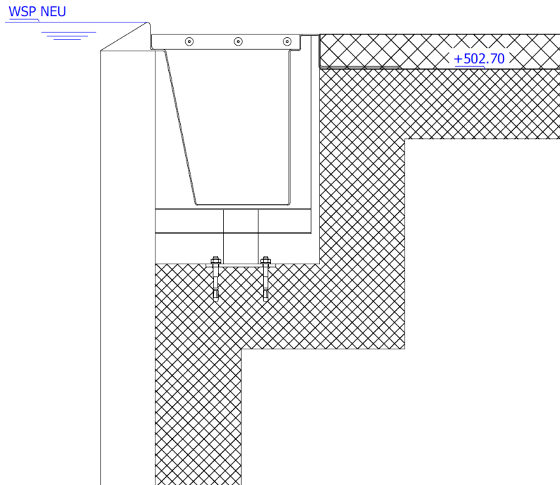
Detail Beckenrand
